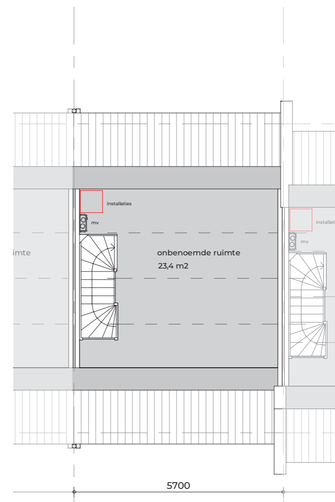
zolder
